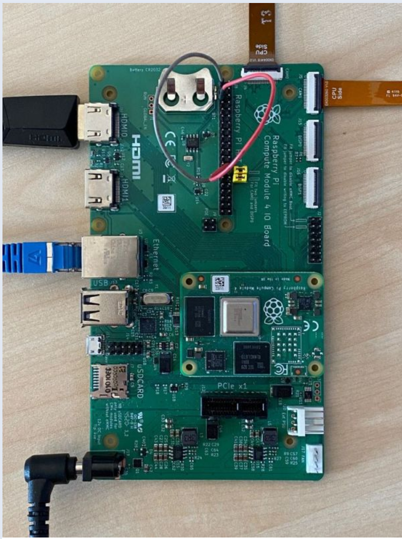
Connection setup
