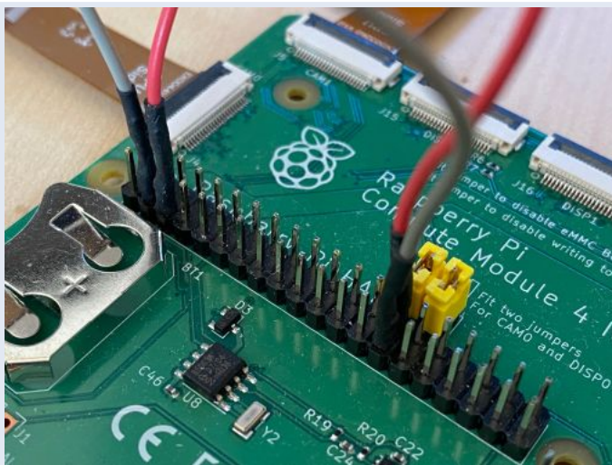
Cable and jumper connections on J8 and J6 headers
