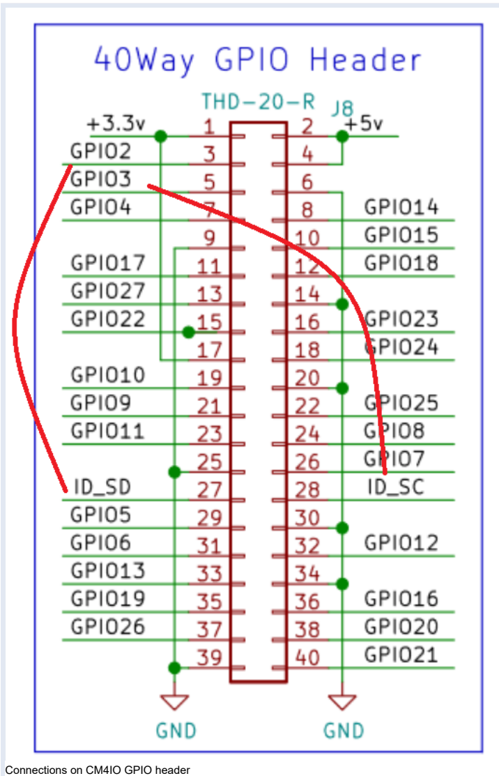
Connections on CM4IO GPIO header
