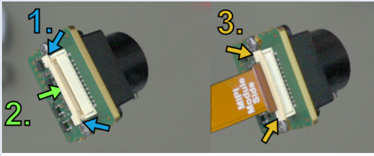
Open the MIPI module socket, put in the cable, close the MIPI module socket
