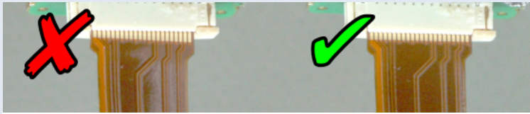
Harmfully angled (left) and good (right) cable fixation
