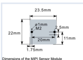
Dimensions of the MIPI Sensor Module
