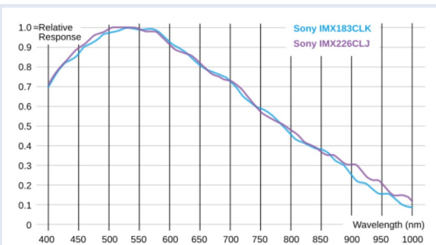
Spectral Curves of selected Monochrome Sensors (2)
