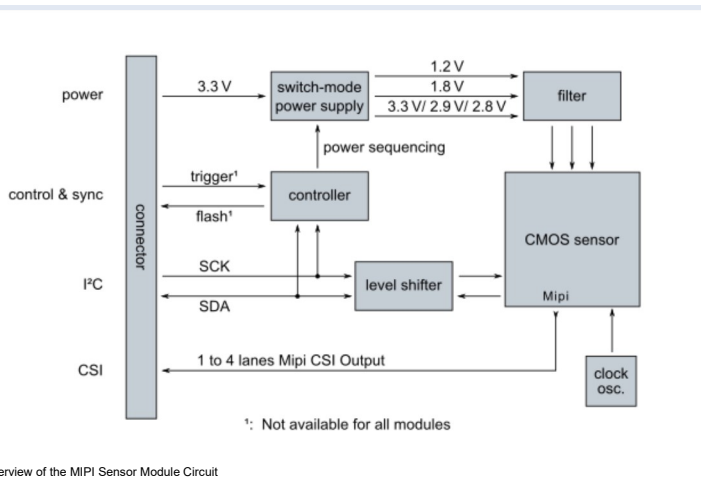
Overview of the MIPI Sensor Module Circuit
