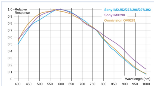
Spectral Curves of selected Monochrome Sensors (1)
