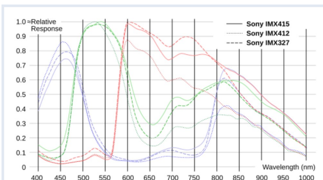
Spectral Curves of selected Color Sensors (1)
