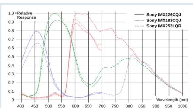
Spectral Curves of selected Color Sensors (2)
