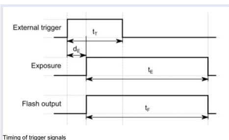
Timing of trigger signals
