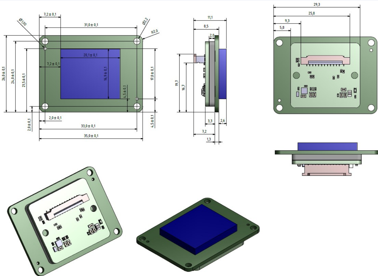
Dimensions of the VC MIPI IMX183
