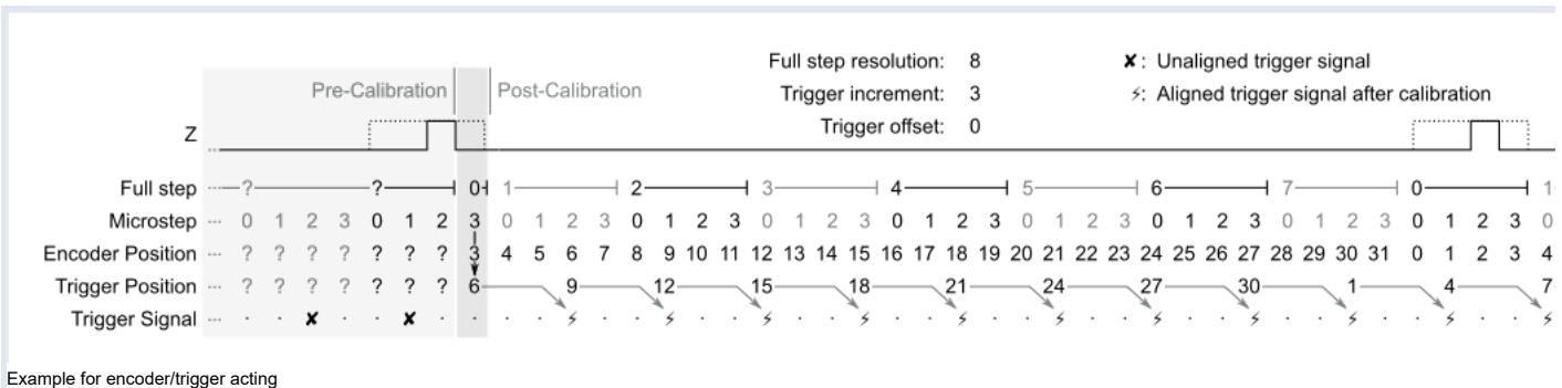
Example for encoder/trigger acting
